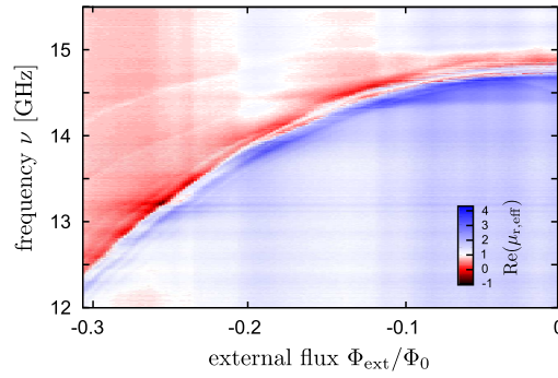
Fig. 3. Real part of the relative magnetic permeability measured at a temperature of 2.3 K.
