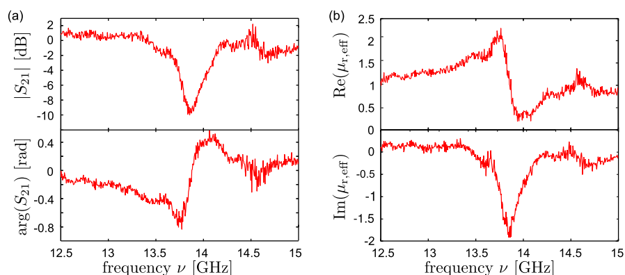
Fig. 1. Corrected version of Fig. 4 in the published paper. Only (b) is affected by the correction of the error. The data are measured at a temperature of 4.2 K.
