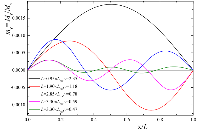
Figure 4. Snapshots of magnetostatic standing waves m_y(x) in L1 0 -FePt FM layer at resonant coupling with Nb/AIO x /Nb LJJ.
