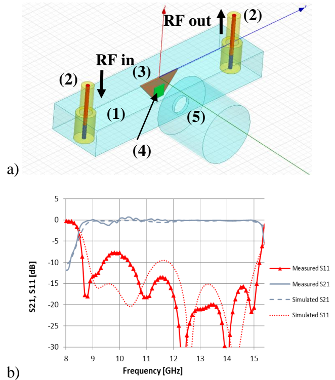
Fig. 1 a) The waveguide chamber used for cryogenic test of RF SQUID metasurface. In the sketch is shown a section of the 19 mm X 9.5 mm waveguide (1). The waveguide section is terminated with the two waveguide-to-coaxial adapters (2) letting the RF signal in and out of the chamber, and the sample mounting plate (3) in the center. When the SQUID array is mounted at the support plate (3) the sample (4) is getting installed inside of the waveguide facing the optical window (5). The window (5) lets in the waveguide the optical probing beam of the Laser Scanning Microscope and is not transparent for the RF probing signal. b) The measured (solid line) and HFSS simulated (dotted line) transmission and reflection coefficients of the test chamber versus frequency of the probing RF signal show the convenience of the developed chamber for the SQUID metasurface characterization in the 8.5 – 15.5 GHz band.
