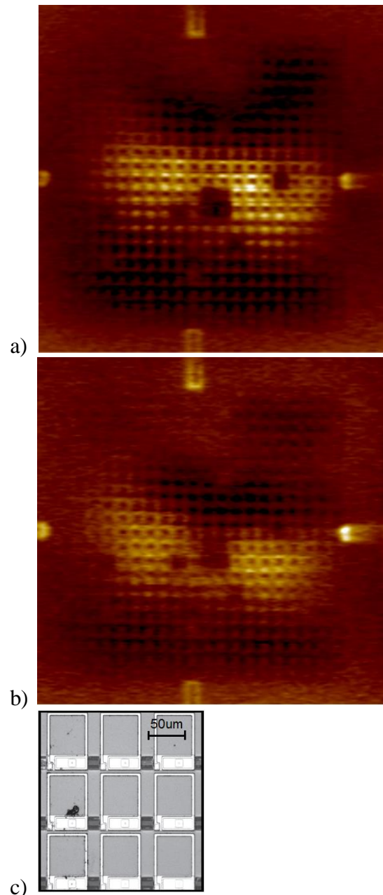
Fig. 3. LSM generated images of the RF currents in the 441 SQUID of the array at the RF frequency close to the maximum resonance frequency of SQUIDs (Fig. 2). The light color coding corresponds to the maximum of LSM response, showing the area with the superconductive circuit with the strongest RF current. (a) LSM data at F max, (b) second LSM run at F max (c) optical image of close up view of 9 SQUIDs in the tested array. The two dark spots in the center of views a) and b) (no RF currents) are likely to be the two defective SQUIDs. One can note that about 50 % of the SQUIDs in the array participating in the resonance (bright color). The remaining question of the resonance modal structure in the SQUID array requires RF phase information unavailable in LSM experiments.
