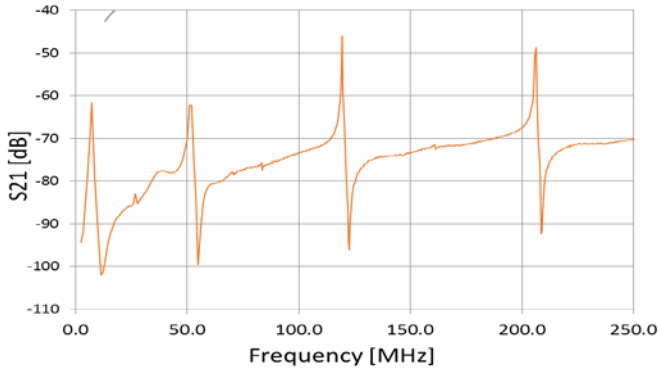
Fig. 3. Measured transmission |S_{21}| of twin-spiral resonators at T=4.5 K in the test setup configuration shown in Fig. 2. The two Archimedean spirals have outer diameter 3 mm and with inner diameter 2.2 mm, 40 turns of Nb wire 5 \mu m wide. The spirals are separated with 300 nm \text{SiO}_2 layer and turning in opposite directions (one clockwise, another counter-clockwise). The opposite winding allows the resonator coupling with RF magnetic field perpendicular to the resonator plane. As result, the coupling of the odd modes ( f_1=7 MHz, f_3=51 MHz and f_5=120 MHz) is stronger, compared to the even modes ( f_2=26 MHz, f_4=82 MHz). The first resonance frequency of the two-spiral resonator ( f_1=7 MHz) is more than 20 lower, compared to the single spiral resonator of the same size [11].
