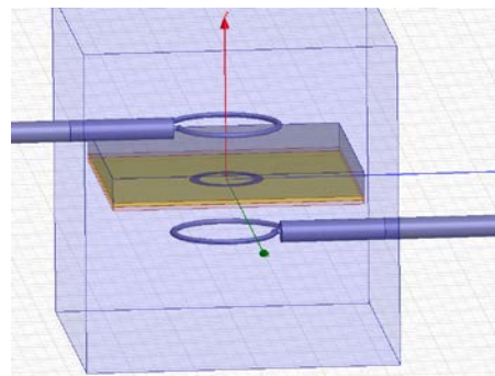
Fig. 2. Experimental RF test setup as simulated numerically in HFSS. A sample of twin-spiral resonator is placed between the two RF loop probes. The two loops probes are weakly magnetically coupled with each other and with the ring shaped resonator. At the resonance frequencies of the two-spiral structure the loop coupling (S21) increases substantially (Fig. 3, 5).
