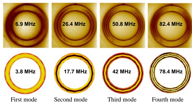
Fig. 5. RF current distribution measured with LSM (above) and HFSS simulated (below) for the first 4 inner modes of the two-spiral resonator. The brighter color corresponds to the higher RF current density. The number of antinodes is equal to the mode number. The capacitive overlap areas do not have pronounced nodal structure in experimental data. The bright background in experimental data is due to a strong photo response in the Si substrate of the tested sample. The measured and calculated resonance frequencies are listed in the middle of each plot.
